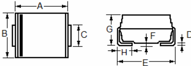
SMC (DO-214AB)
