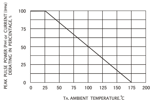
FIG. 2-PULSE DERATING CURVE
