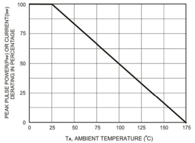
FIG.2-PULSE DERATING CURVE
