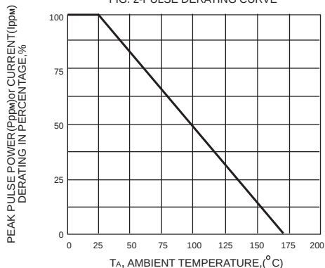
FIG. 2-PULSE DERATING CURVE
