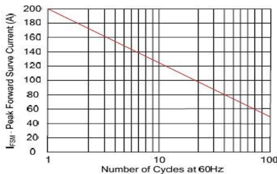
Figure 6. Maximum Non-Repetitive Forward
