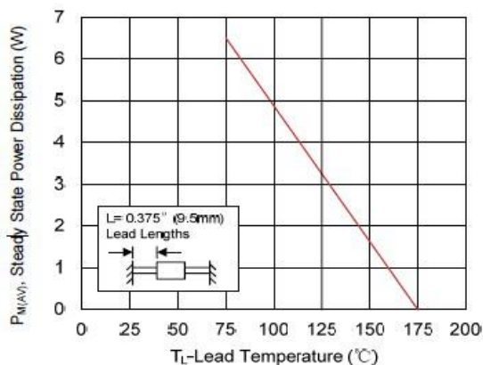
Figure 5. Steady State Power Dissipation Derating Curve Surge Current Uni-Directional Only
