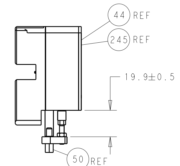
HOLDDOWN SET-UP
