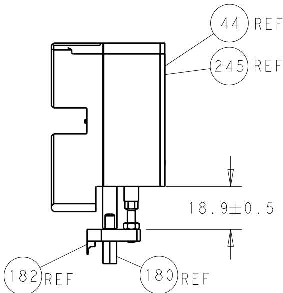
HOLDDOWN SET-UP
