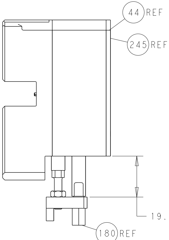
HOLDDOWN SET-UP
