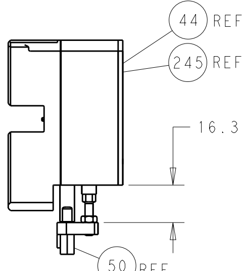
HOLDDOWN SET-UP
