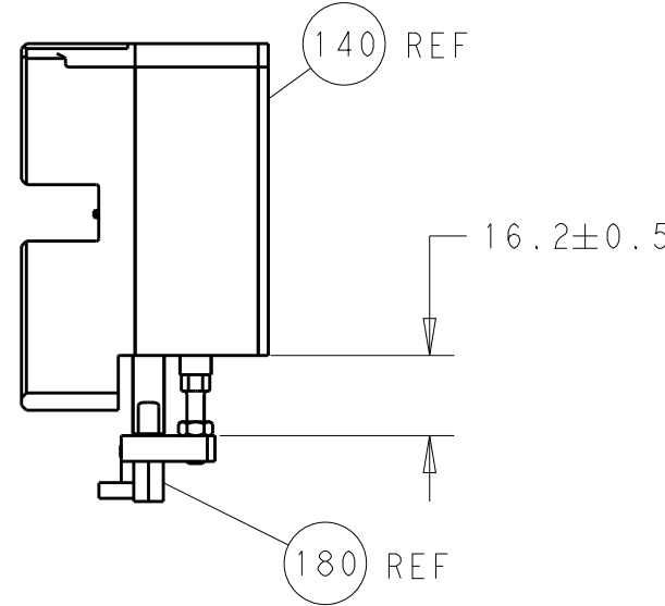
HOLDDOWN SET-UP
