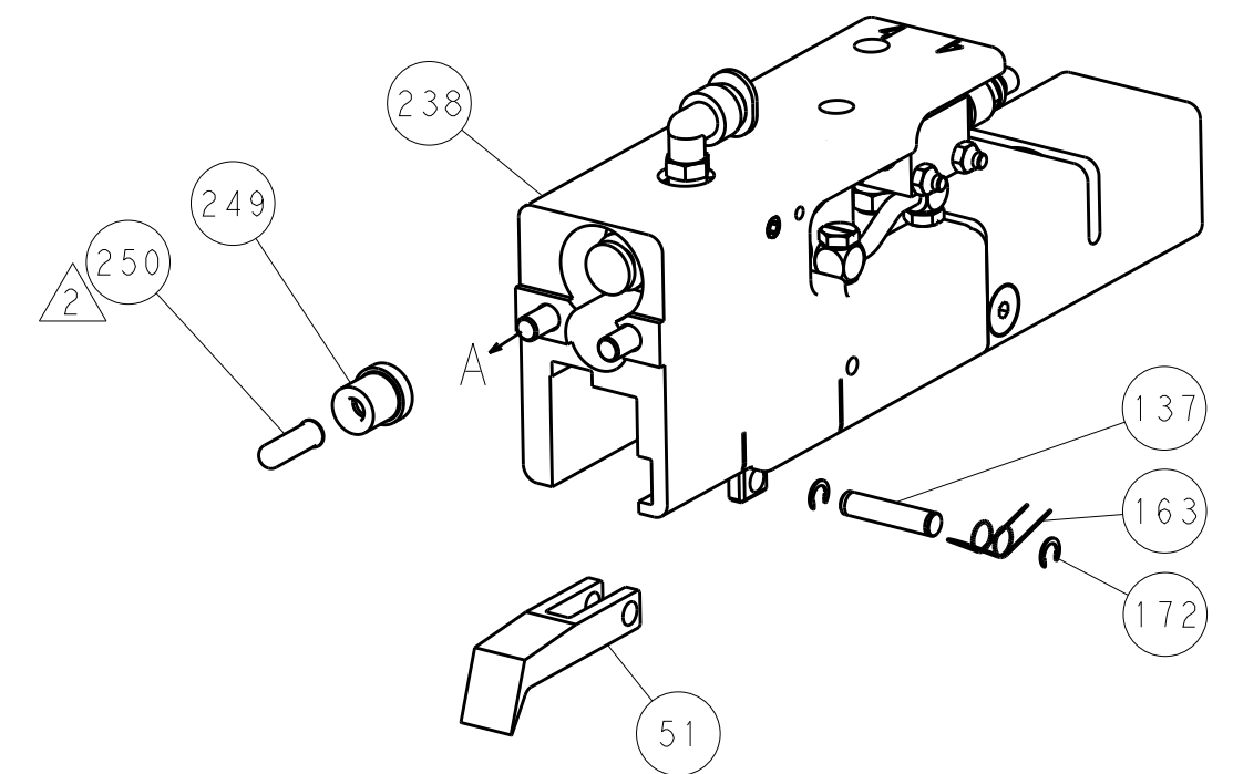
PNEUMATIC
