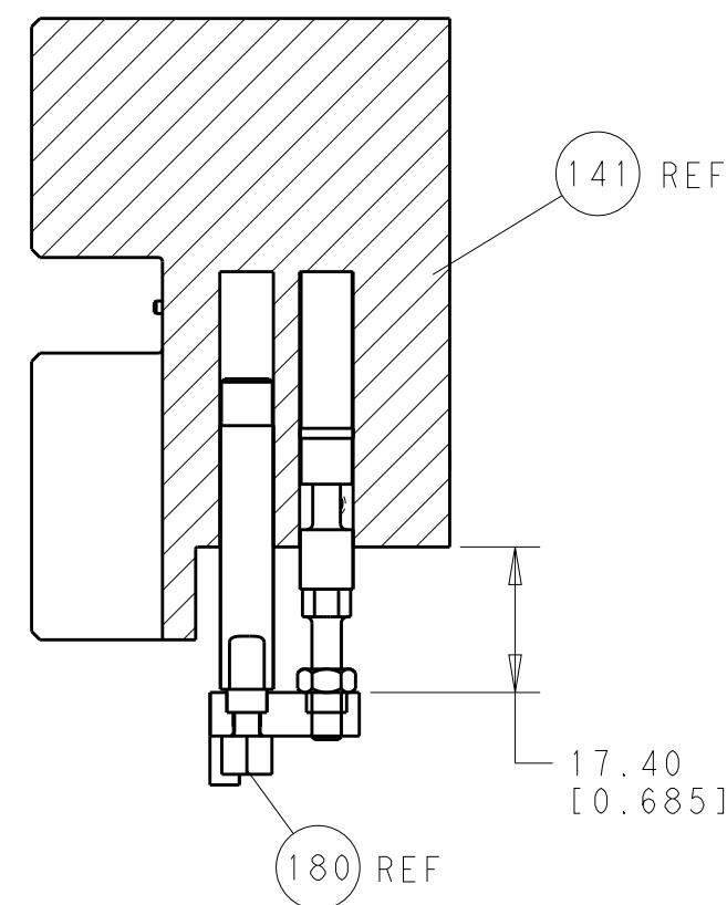
HOLDDOWN SET-UP
