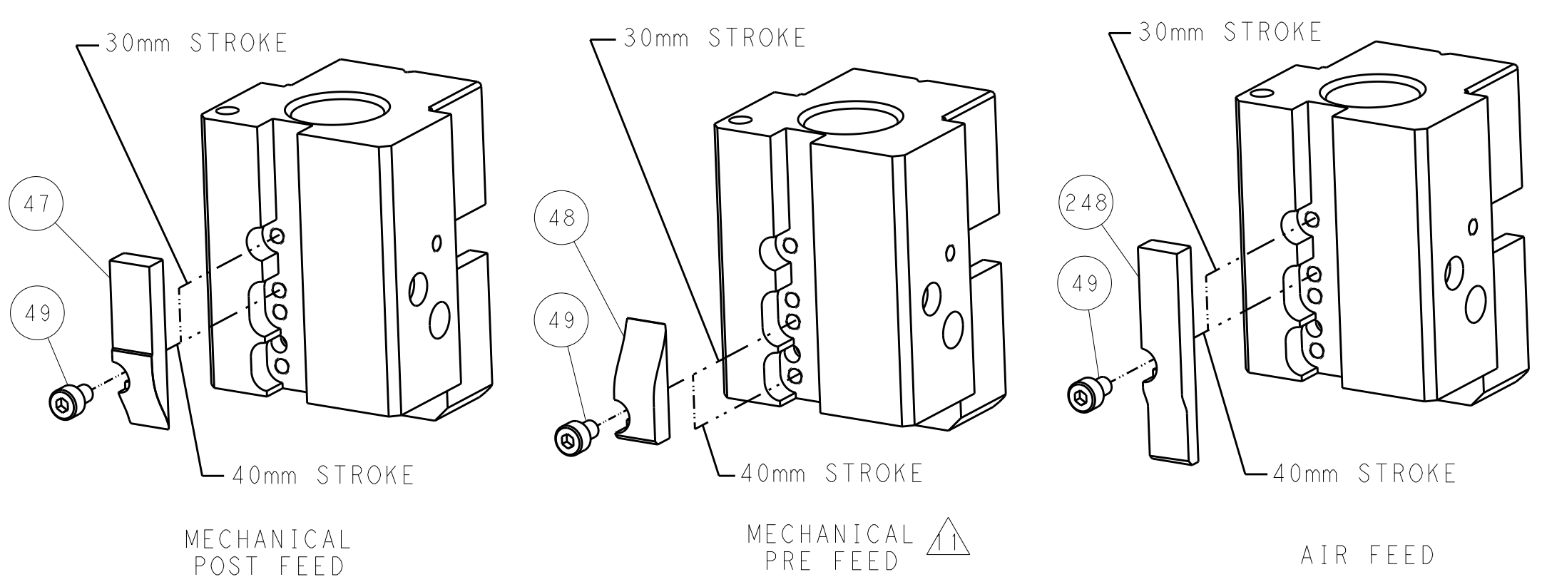
CAM POSITIONS
