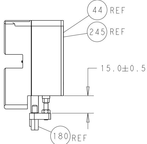
HOLDDOWN SET-UP
