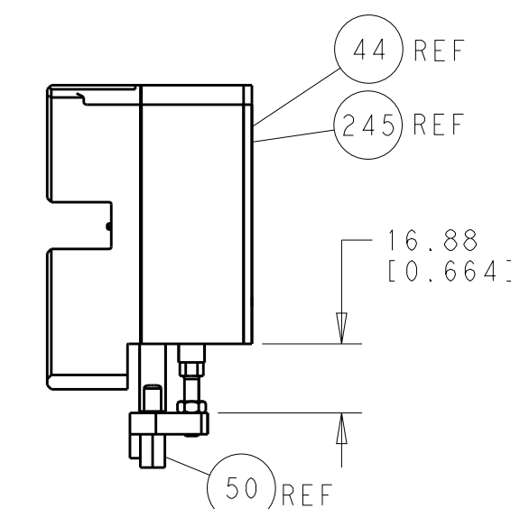
HOLDDOWN SET-UP
