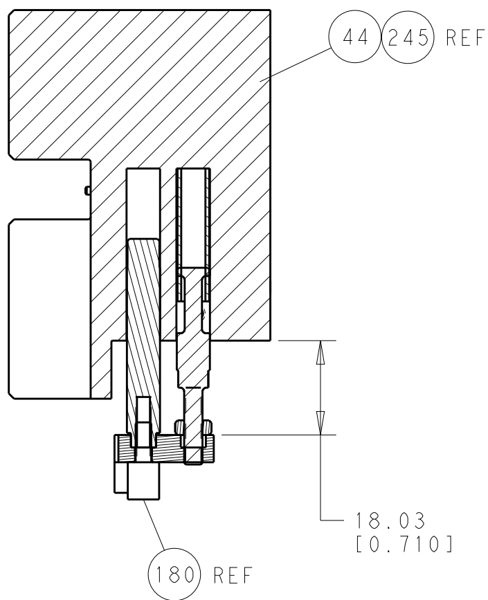
HOLDDOWN SET-UP
