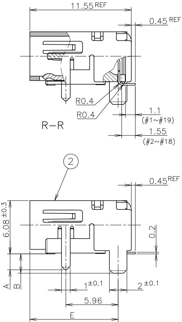
CONNECTOR WITHOUT FLANGE TYPE
