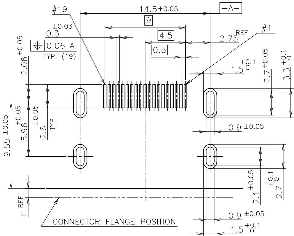
P.C.B LAYOUT SHOWN AS CONNECTOR MOUNTING SIDE TOLERANCE: NON-CUMULATIVE (REFERENCE)
