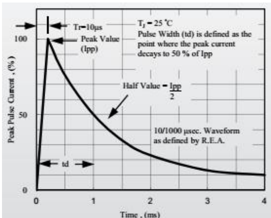
Figure 5- Pulse Waveform
