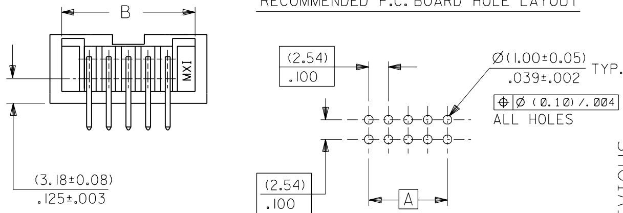
RECOMMENDED P.C. BOARD HOLE LAYOUT
