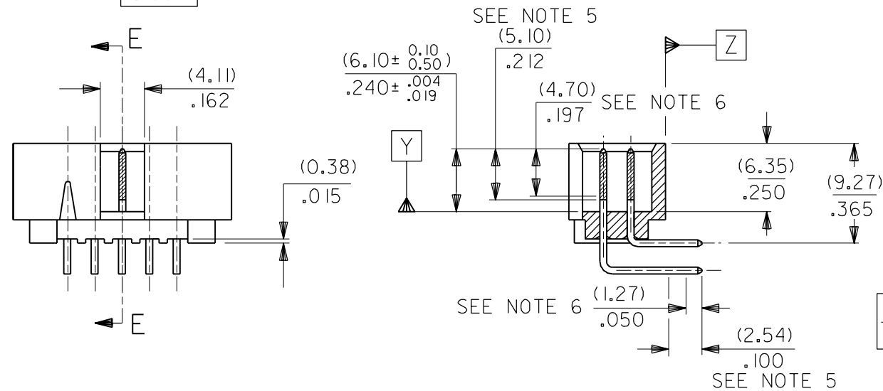
SECTION E-E
