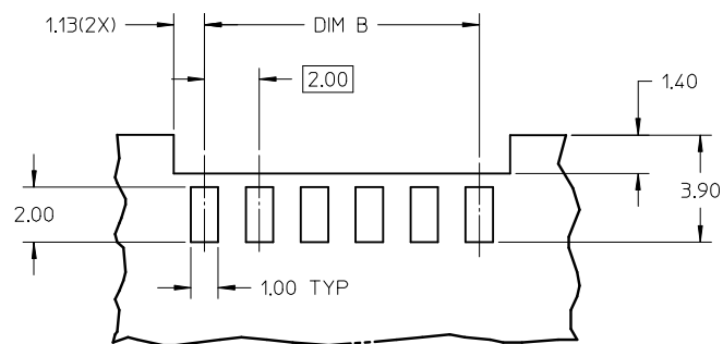
RECOMMENDED PCB PATTERN (PATTERN TYPICAL BOTH SIDES)
