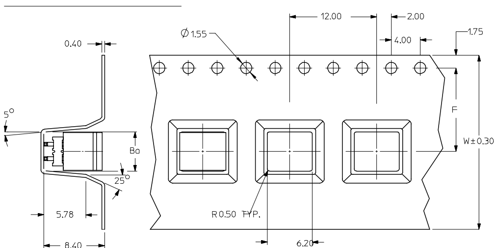
EMBOSSED CARRIER TAPE TYPE "C"
