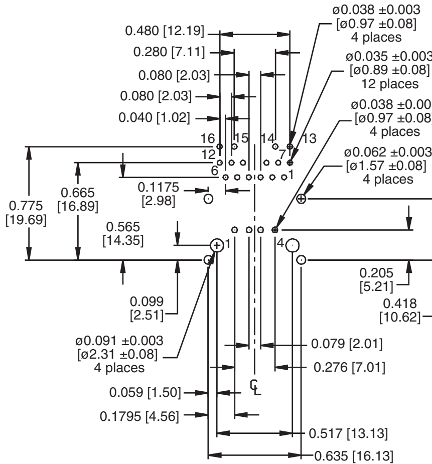
Suggested PCB Pad Layout Component Side View
