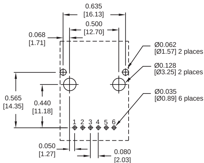
Suggested PCB Pad Layout
