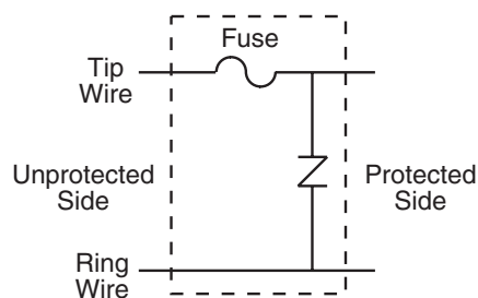
2-Wire Protection
