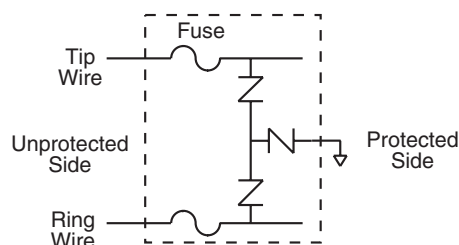
"Y" Inter-wire and Ground Protection
