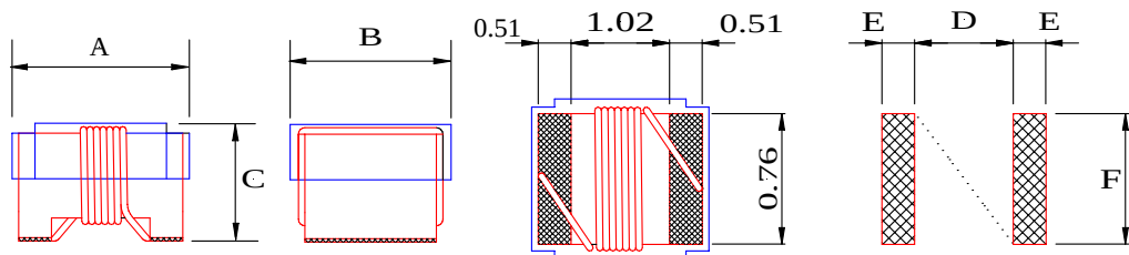
Land Pattern
