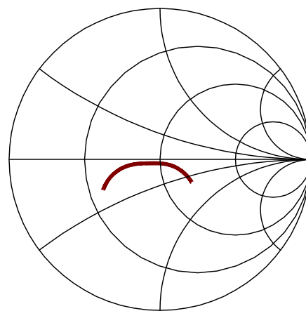
S22 (63.26-73.26 MHz)
