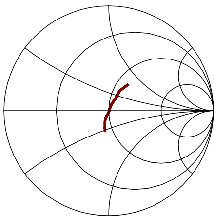
S11 (63.26-73.26 MHz)
