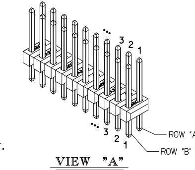
SECTION Z-Z - RETENTION PIN DETAIL 2 CONTACTS LOCATED ON CENTER OF SAME ROW (SEE NOTE 6)
