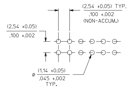
PCB LAYOUT: COMPONENT SIDE TYPICAL PCB THICKNESS: (1.57)/.062
