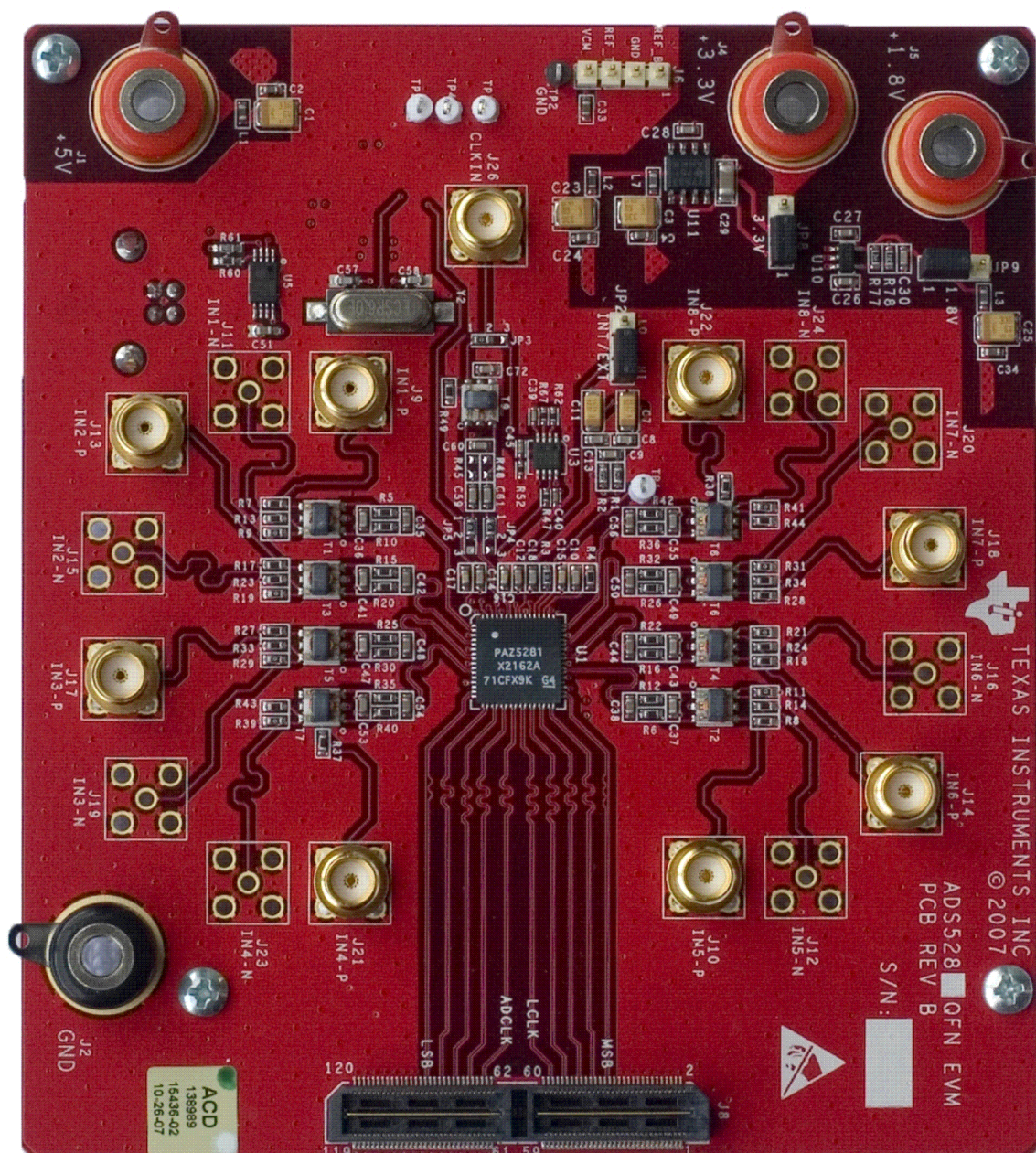
Figure 1. ADS5281 EVM
