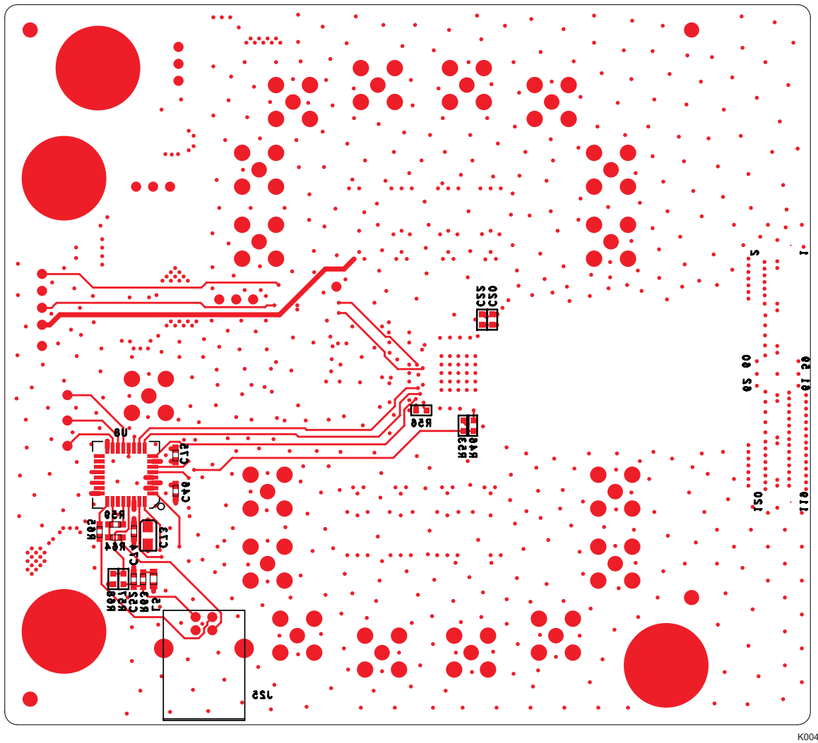
Figure 6. Bottom Silkscreen
