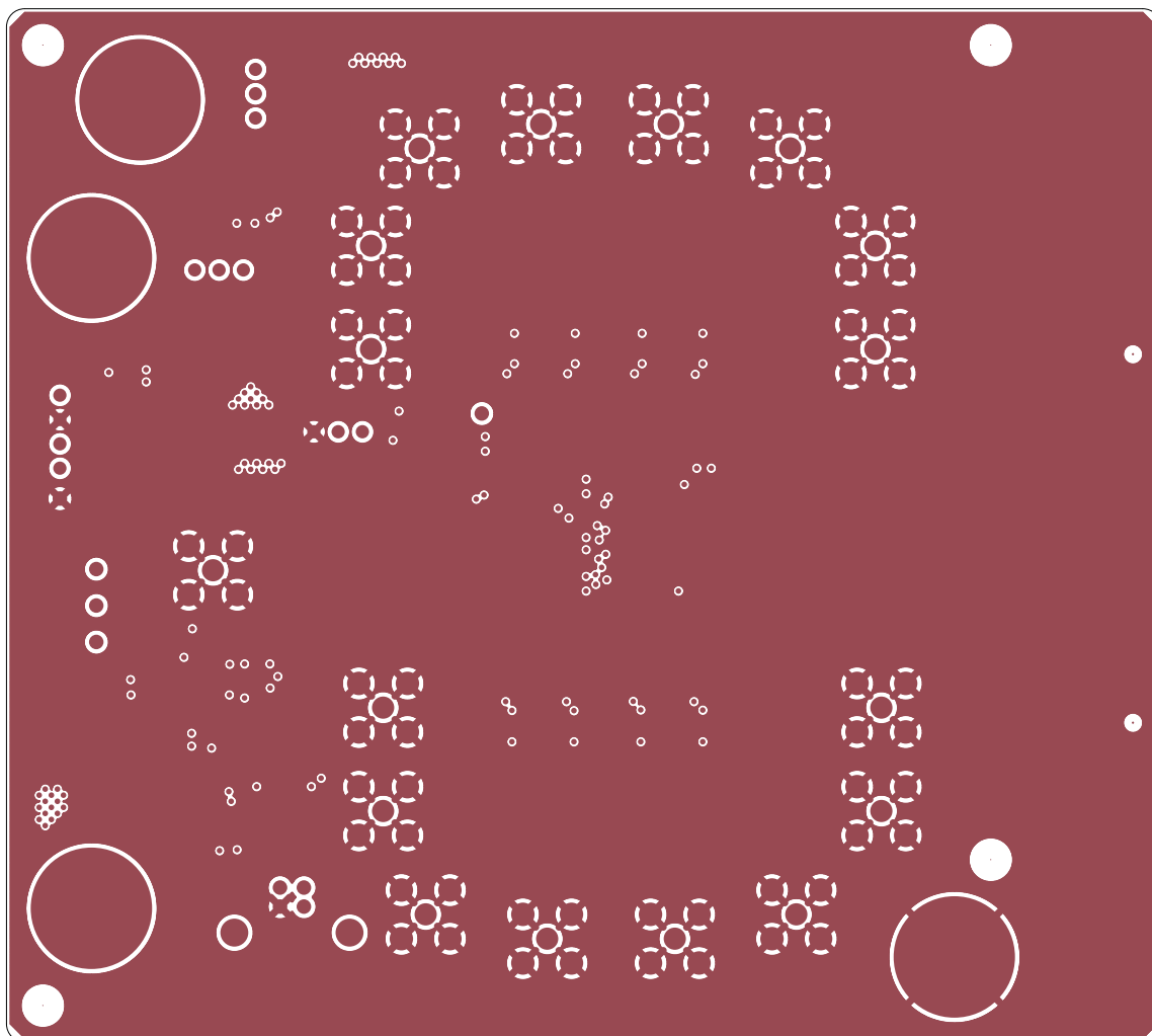
Figure 4. Ground Plane
