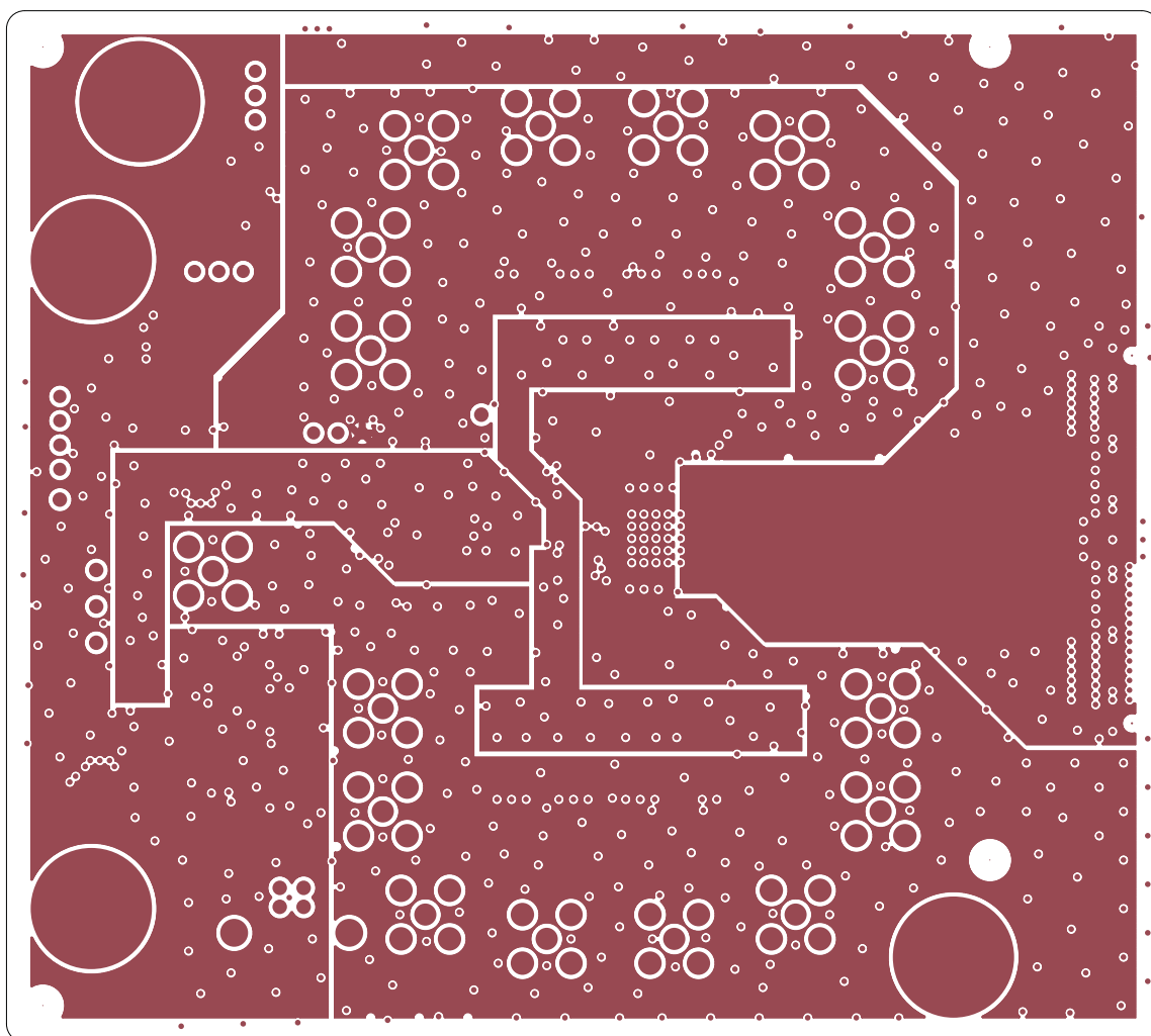
Figure 5. Power Plane
