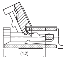
SEC A - A"
