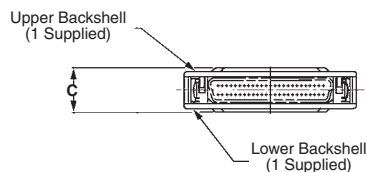
Style B Straight Exit with Latches
