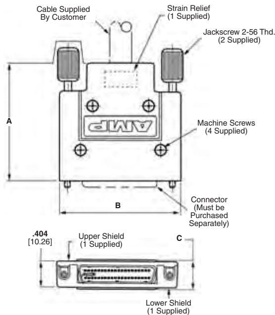
Style B Straight Exit Male Jackscrews
