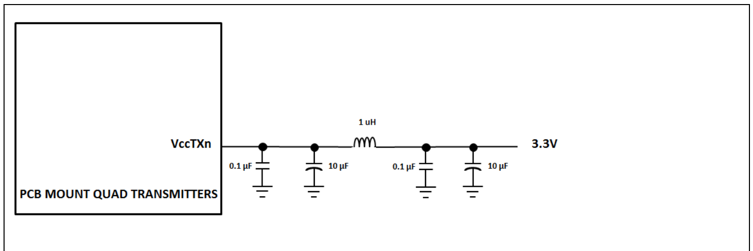
FIGURE 5 – RECOMMENDED HOST BOARD POWER SUPPLY FILTERING CIRCUIT SINGLE TRANSMITTER SHOWN (X4 TRANSMITTERS PER MODULE)
