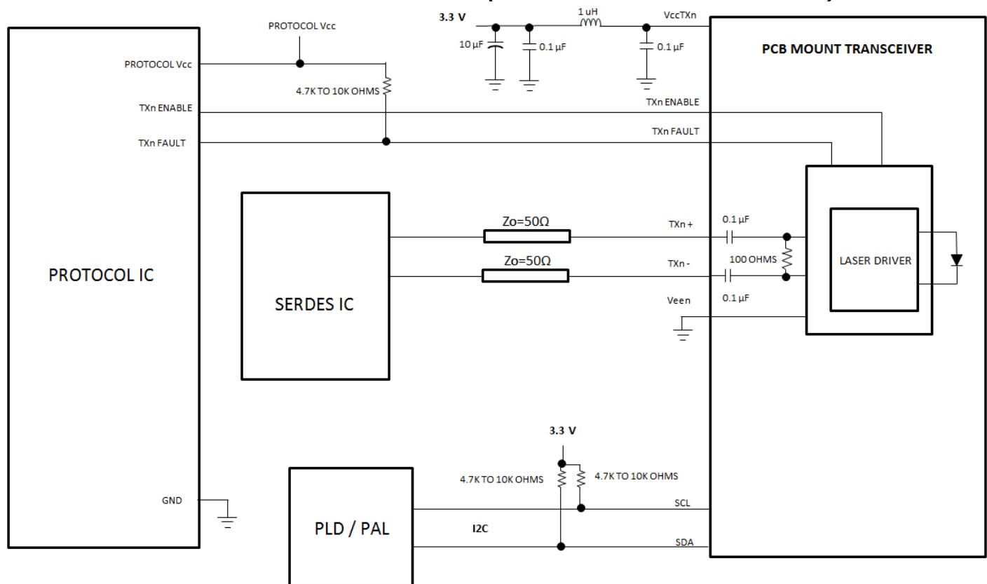
FIGURE 3 – HOST BOARD RECOMMENDED SCHEMATIC SINGLE TRANSMITTER SHOWN (X4 TRANSMITTERS PER MODULE)
