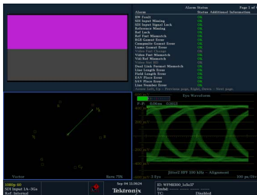
+25C, -17 dBm at the receiver 050-332
