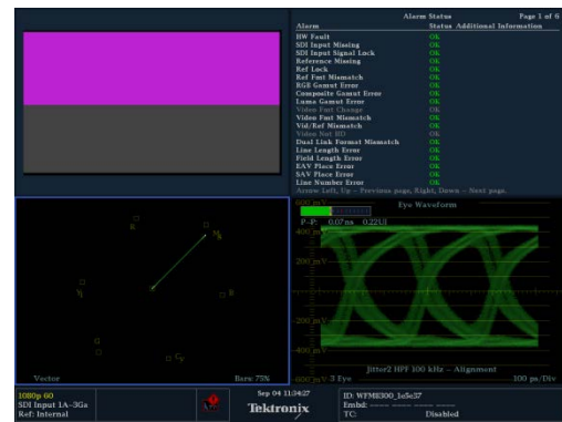
+25C, -5 dBm at receiver 050-332
