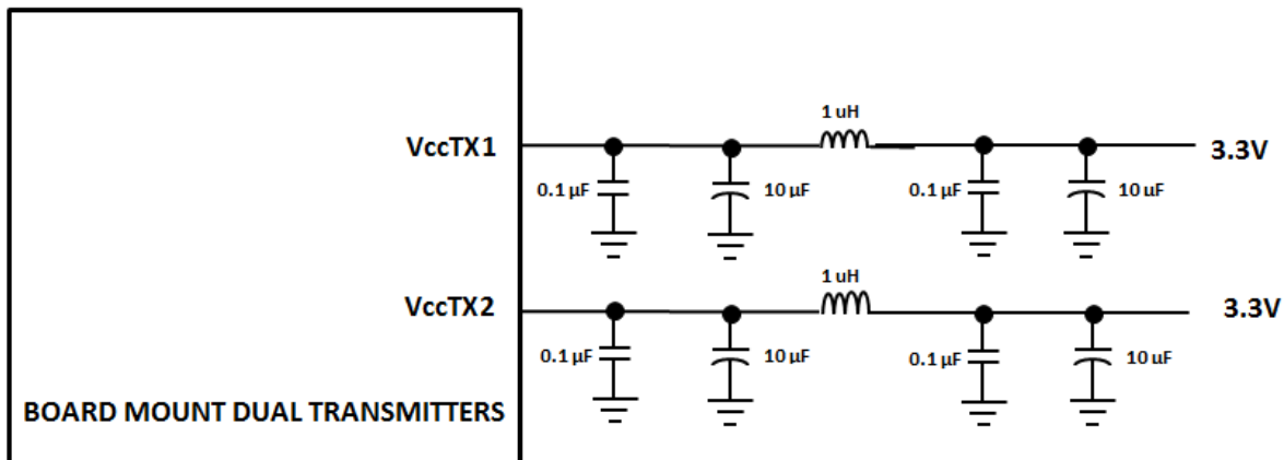
FIGURE 5 RECOMMENDED HOST BOARD POWER SUPPLY FILTERING CIRCUIT
