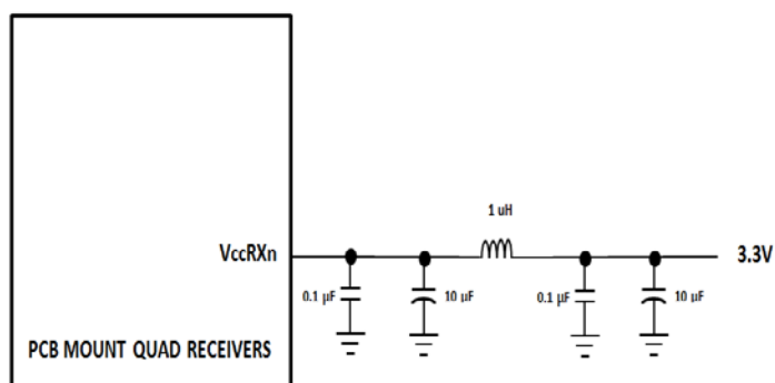
FIGURE 5 RECOMMENDED HOST BOARD POWER SUPPLY FILTERING CIRCUIT
