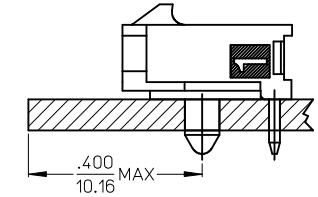
LOCATION DETAIL (SEE NOTE #6)
