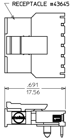
MATED MICRO FIT CONNECTOR
