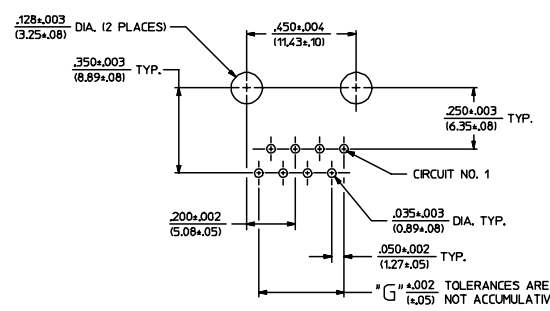
P.C. BOARD LAYOUT FOR CONNECTOR SIZE 8
