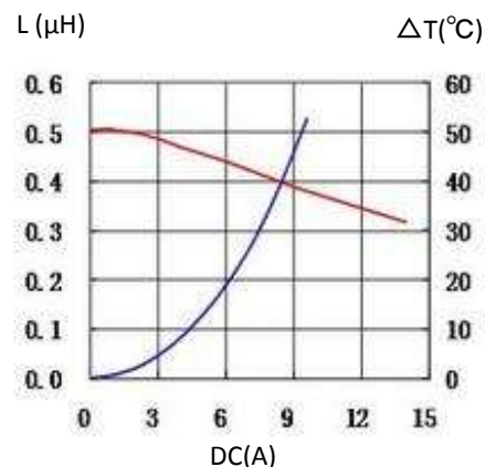
3. 0415CDMCCDS-R47MC
