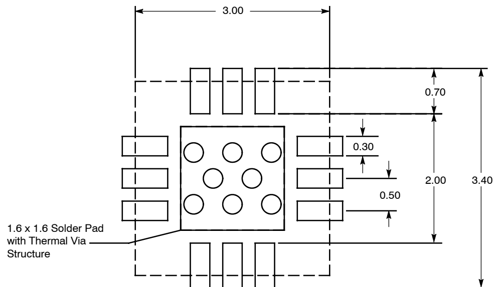
Figure 7. PCB Pad Layout for QFN 3x3
