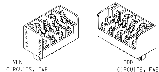
NUMBER OF CIRCUITS "A" DIM. "B" DIM. MATERIAL NUMBER 03 16.51 1.6501 7.62 1.3001 399300303 04 20.32 1.8001 11.43 1.4501 399300304 05 24.13 1.9501 15.24 1.6001 399300305 06 27.94 1.1.1001 19.05 1.7501 399300306 07 31.75 1.1.2501 22.86 1.9001 399300307 08 35.56 1.1.4001 26.67 1.1.0501 399300308 09 39.37 1.1.5501 30.48 1.1.2001 399300309 10 43.18 1.1.7001 34.29 1.1.3501 399300310 11 46.99 1.1.8501 38.10 1.1.5001 399300311 12 50.80 1.2.0001 41.91 1.1.6501 399300312 13 54.61 1.2.1501 45.72 1.1.8001 399300313 14 58.42 1.2.3001 49.53 1.1.9501 399300314 15 62.23 1.2.4501 53.34 1.2.1001 399300315 16 66.04 1.2.6001 57.15 1.2.2501 399300316 17 69.85 1.2.7501 60.96 1.2.4001 399300317 18 73.66 1.2.9001 64.77 1.2.5501 399300318 19 77.47 1.3.0501 68.58 1.2.7001 399300319 20 81.28 1.3.2001 72.39 1.2.8501 399300320 21 85.09 1.3.3501 76.20 1.3.0001 399300321
