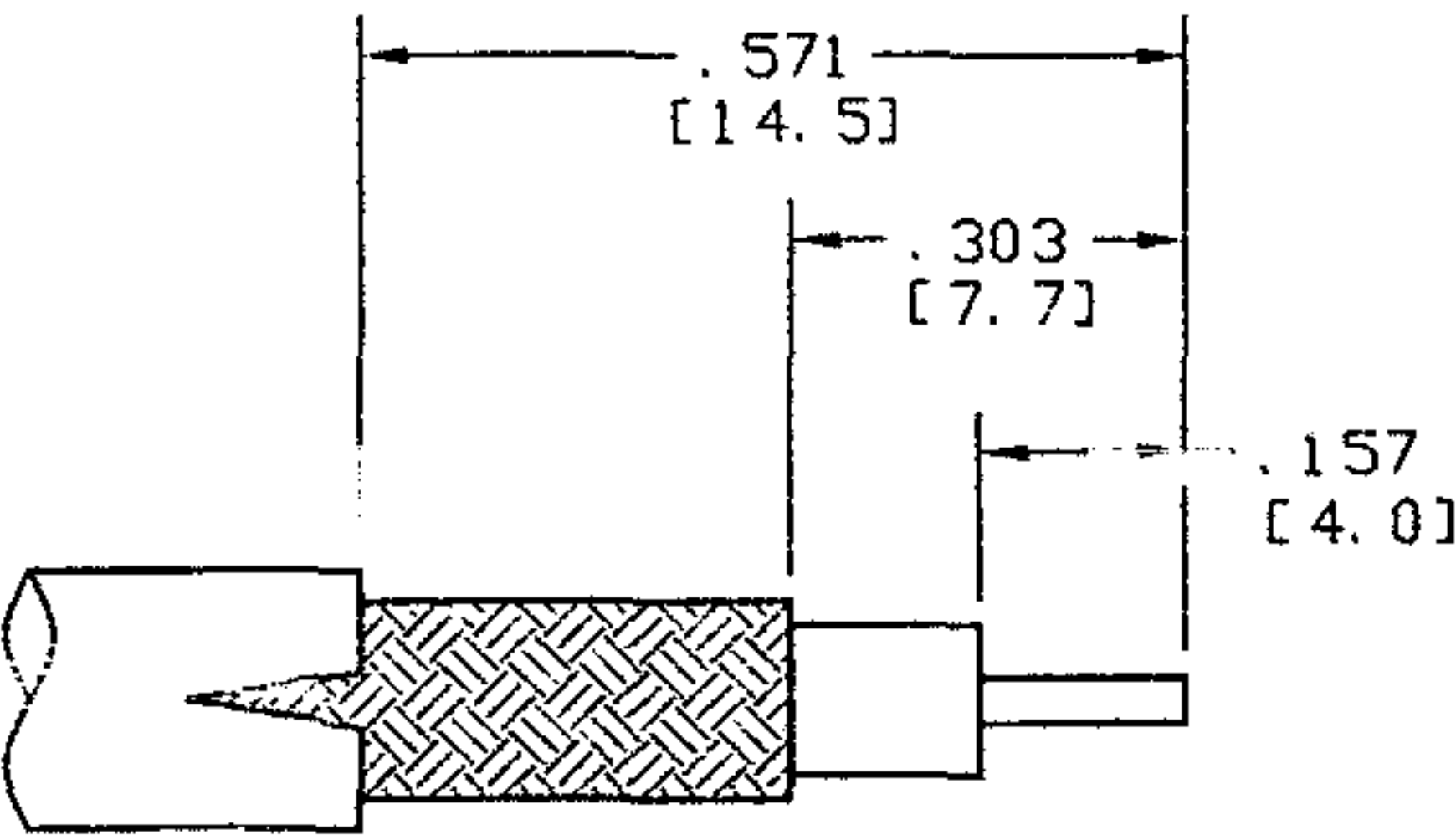
RECOMMENDED CABLE STRIPPING DIM'S
