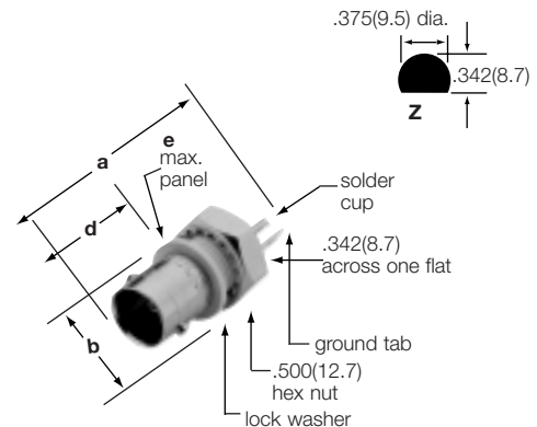
75Ω BNC Receptacle (J) Isolated from Panel with Solder Cup & Ground Tab 31-10-75 31-10-75 RFXG2
