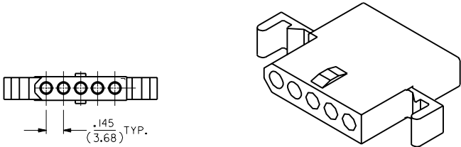
RECEPTACLE HOUSING SHOWN WITH STANDARD EARS
