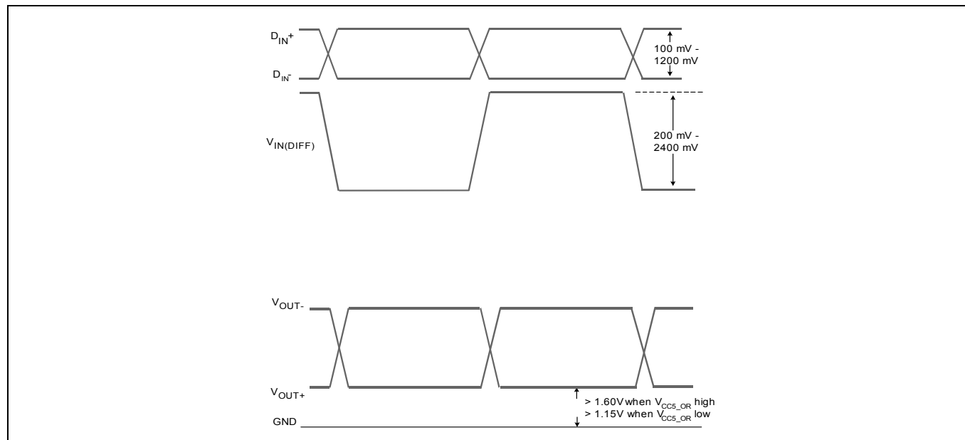
Figure 1-1. Relationship between Data Inputs and Modulation Outputs
