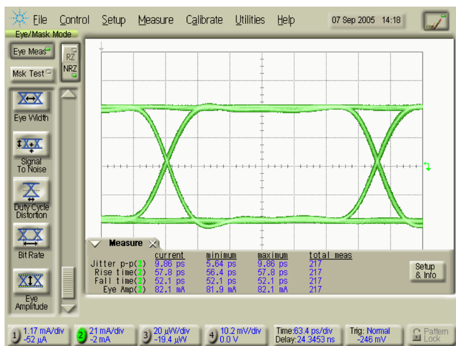
Figure 3-2. 2.5Gbps Electrical Eye Diagram
