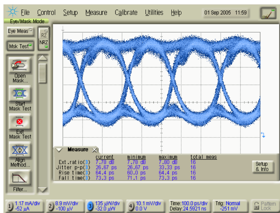
Figure 3-4. 4.25Gbps Unfiltered Optical Eye Diagram with Archcom AC3460 Laser
