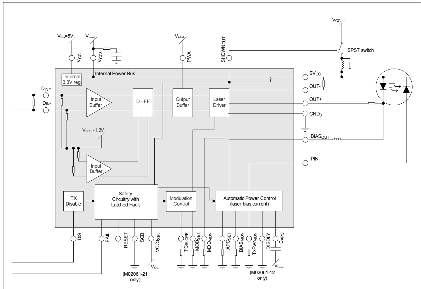
Figure 4-2. Application Diagram, VCC = 5V Laser DC Coupled Example
