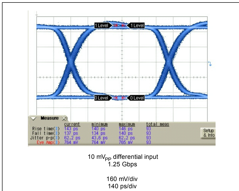
Figure 1-2. M02046 on an MC2046 EVM
