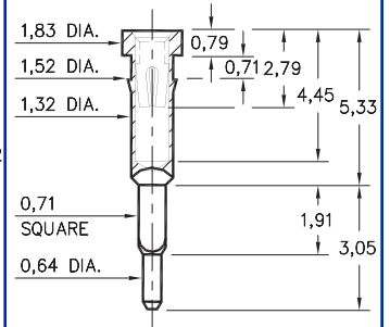
9970-0-15-XX-30-XX-04-0 Square press-fit for 0,81 ±0,05 plated thru hole
