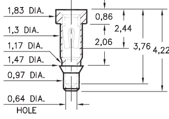
1434-0-15-XX-30-XX-10-0 Press-fit in 1,4 mounting hole
