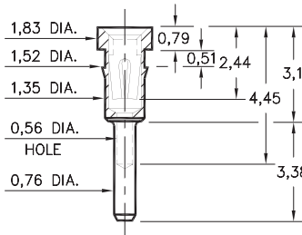
8427-0-15-XX-30-XX-04-0 Press-fit in 1,45 mounting hole
