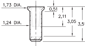
0680-0-15-XX-32-XX-10-0 Solder mount in 1,3 min. mounting hole Also available on 16mm wide carrier tape: 1,700 parts per 330mm reel. Order as: 0680-0-57-XX-32-XX-10-0
