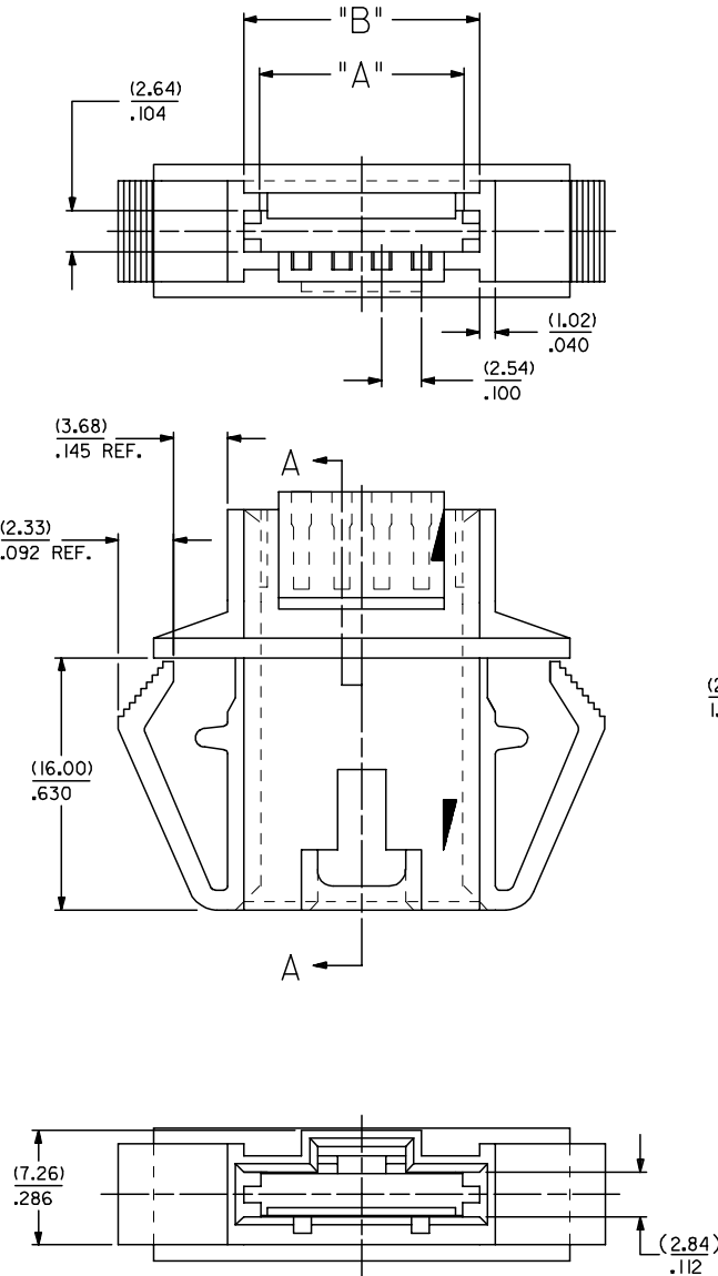
2 CIRCUIT
