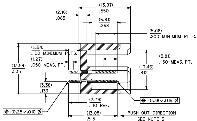
SECTION W-W
