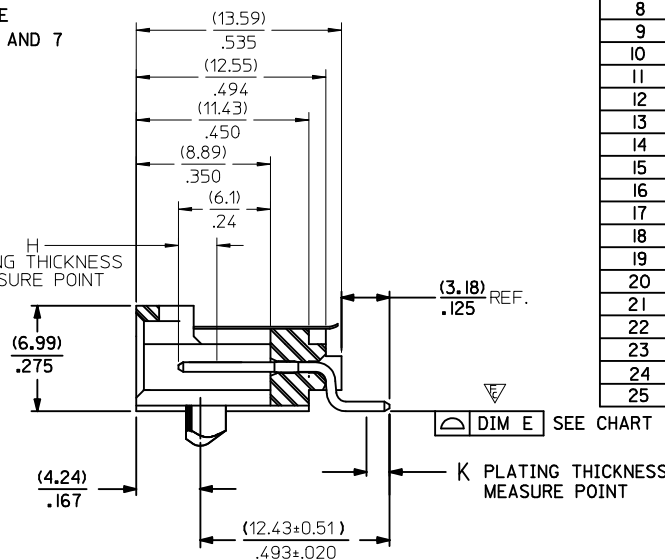
SECTION F-F
