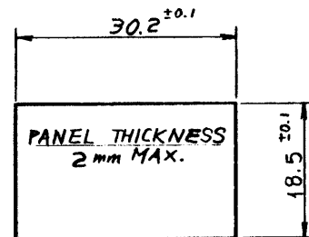
MOUNTING HOLE DETAIL (SCALE 1:1)
