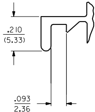
DETAIL 3
